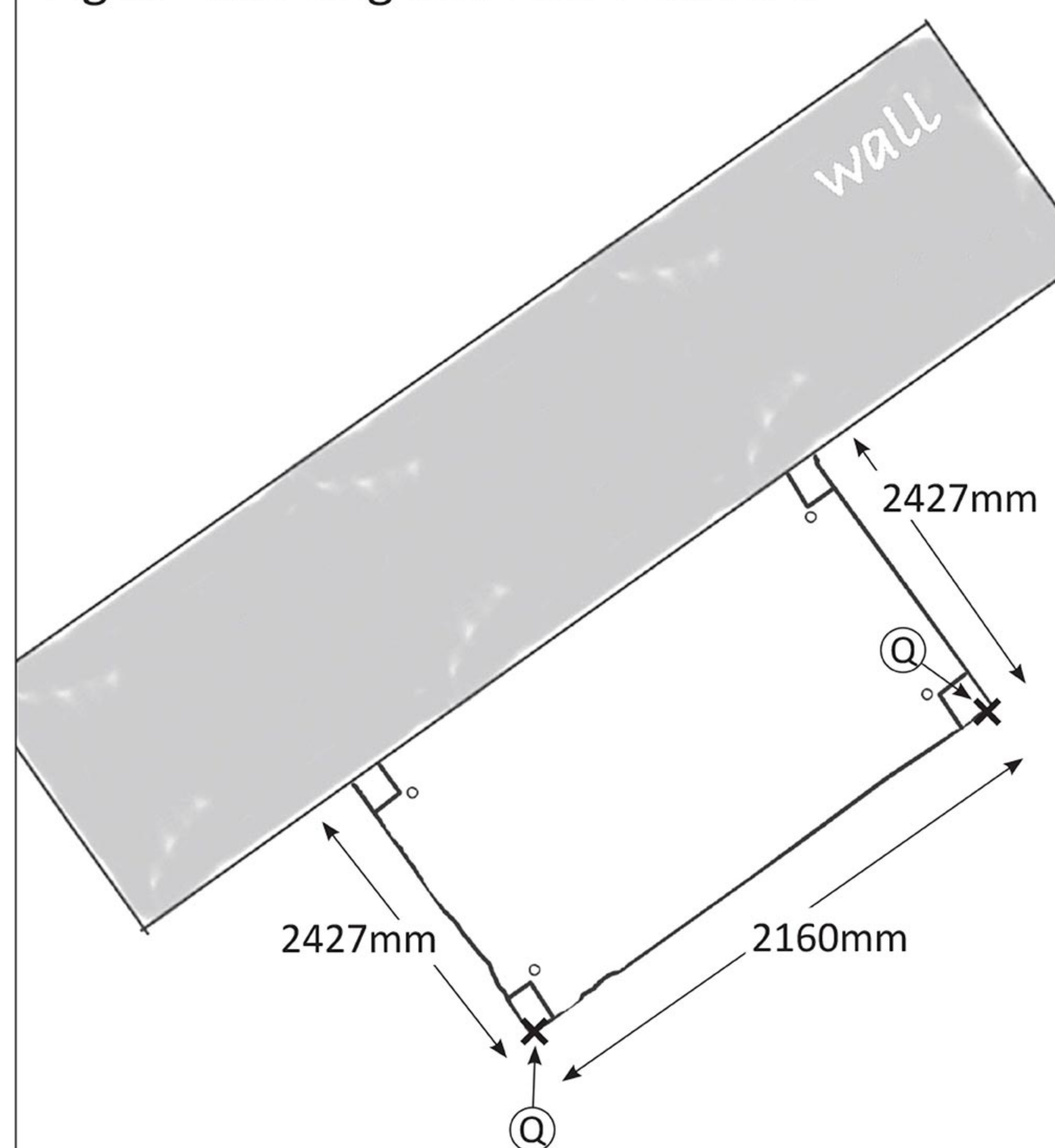
Fig 1. - Marking Out Post Positions
