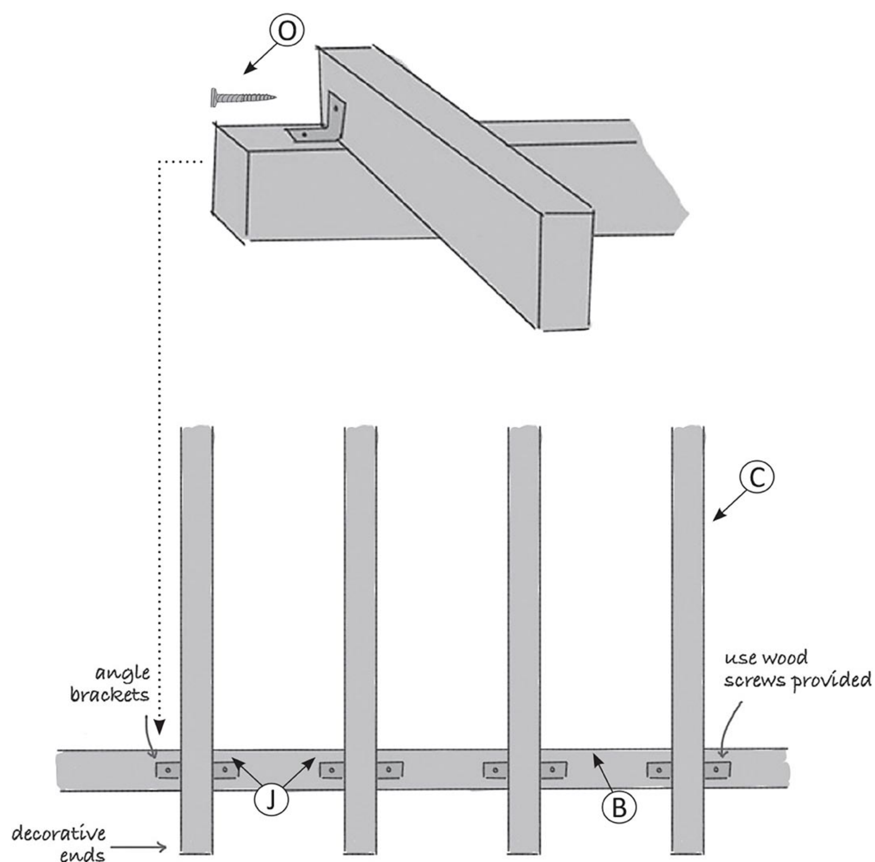
Fig 6. - Attaching Cross Rafter to Main Beam
