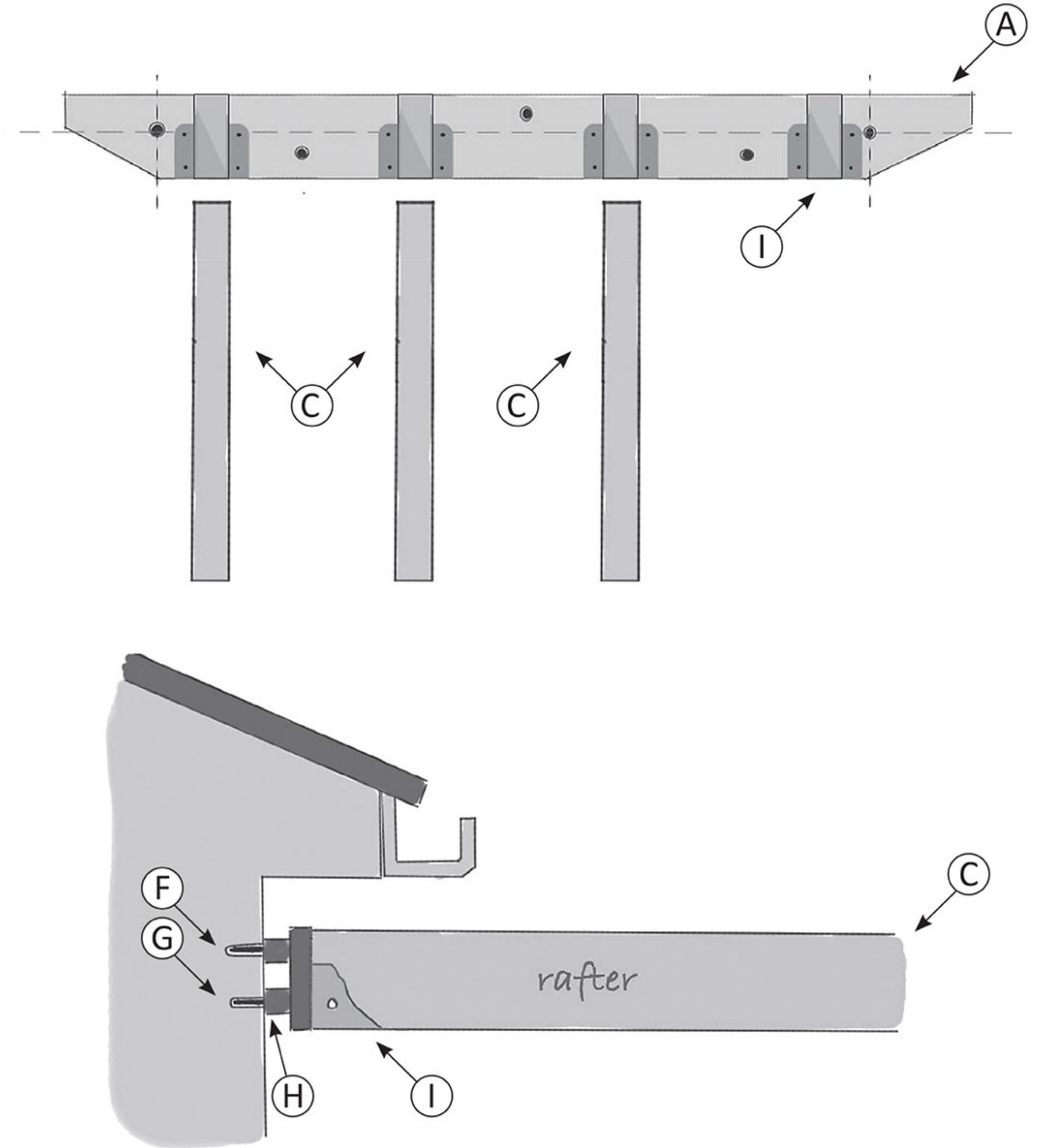
Fig 6. - Attaching Cross Rafter to Ledger Board
