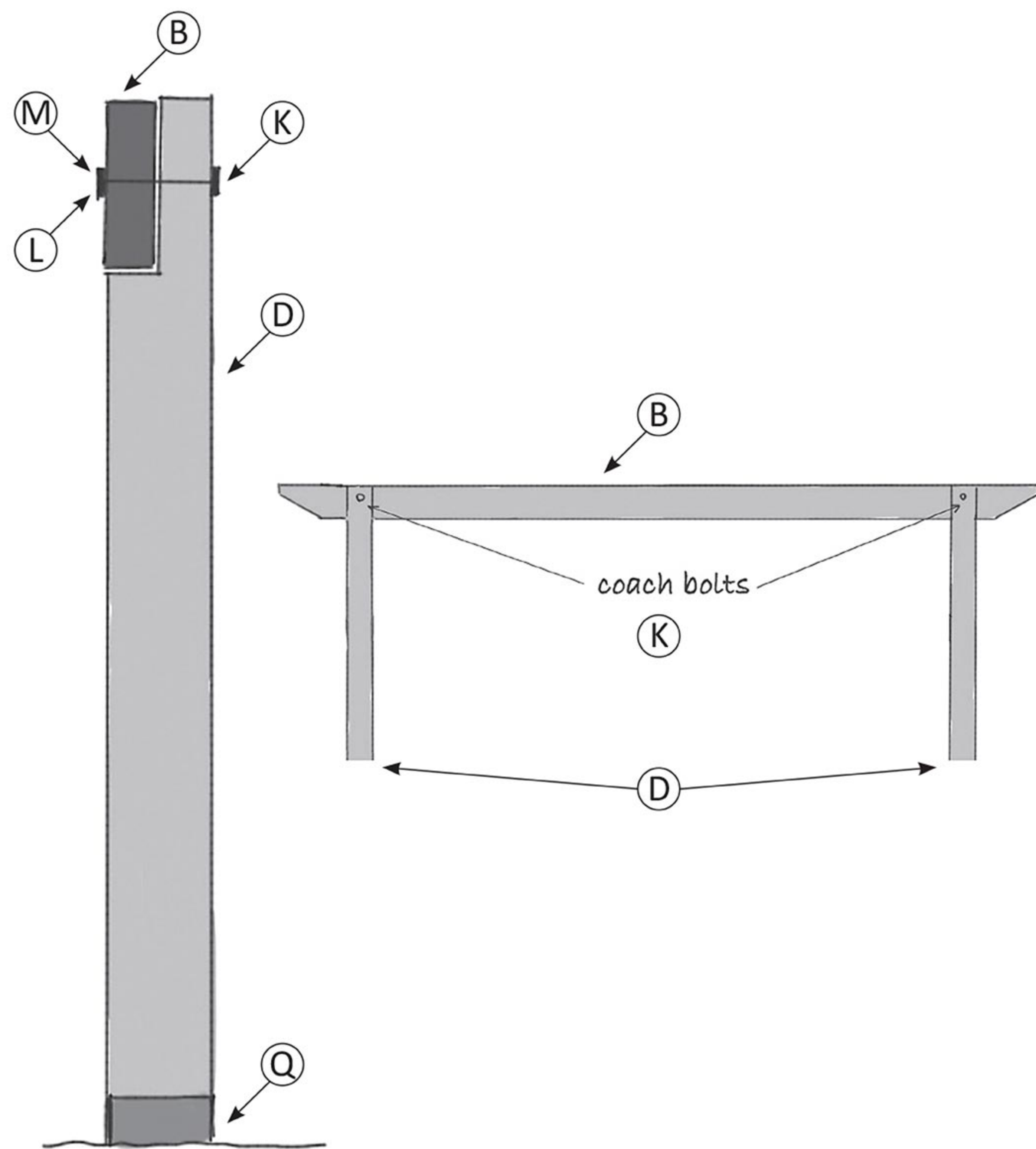
Fig 5. - Fitting Main Beam
